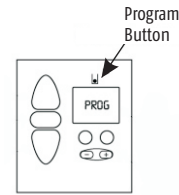
Chronis RTS Timer with cover removed
